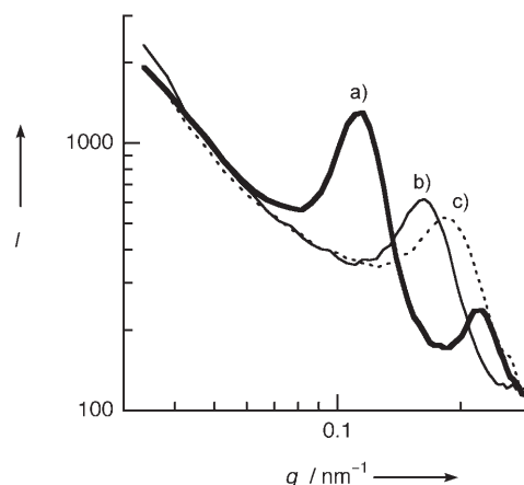
Figure 4. Small-angle neutron scattering (SANS) profiles of hectorite–niobate colloids. The colloids contain 62.0 \text{ g L}^{-1} of niobate nanosheets and a) 0, b) 10.0, and c) 17.5 \text{ g L}^{-1} of hectorite nanosheets.
